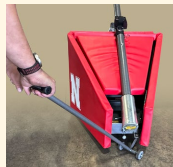
Transport Dolly
